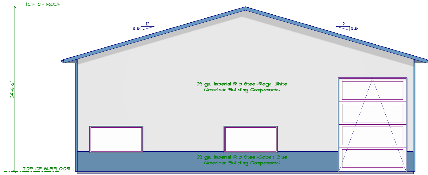
NORTH ELEVATION
